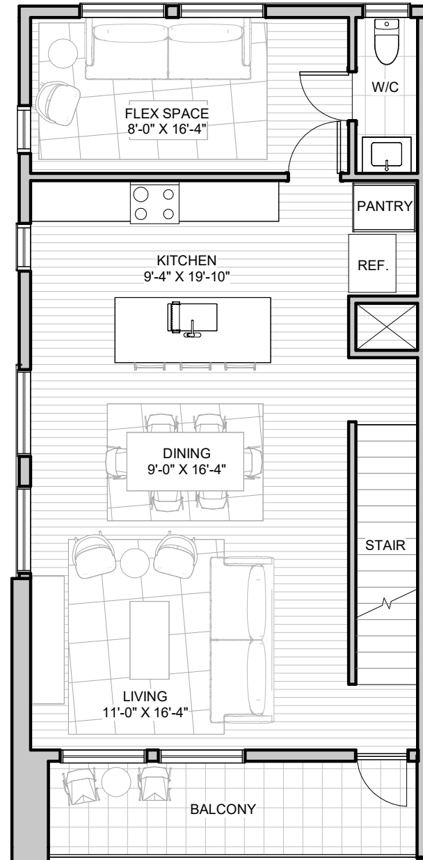
LEVEL 2
